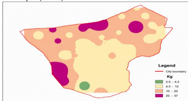
4-rasm. Termiz shahri hududi bo'yicha K_g koeffitsientining taqsimlanish xaritasi
